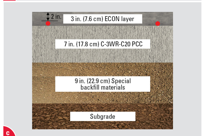
ECON HPS test site: (a) construction location, (b) plan view, and (c) cross-section view
