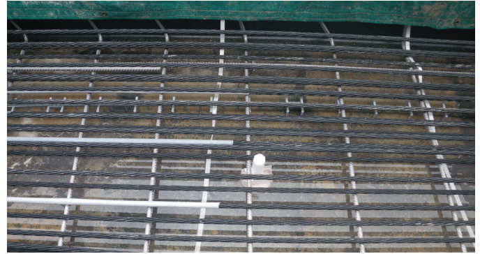
▶ Prestressed concrete box beam casting bed with the CFCC strand, strand debonding plastic sleeves, and the bottom stainless steel U-rebars used for shear reinforcement installed in place near the beam end.
